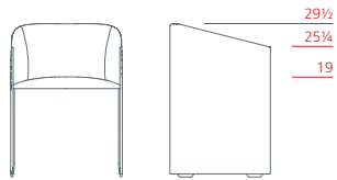
Tall armchair on feet 1PL6012: L 22 D 20 H 29½
