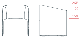
Lounge armchair on feet 1PL6022: L 22 D 22¾ H 26½
